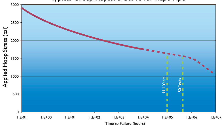
Typical Creep Rupture Curve for hdpe Pipe
