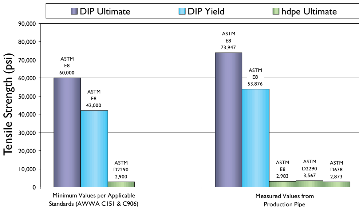
FIGURE I Tensile Strength
